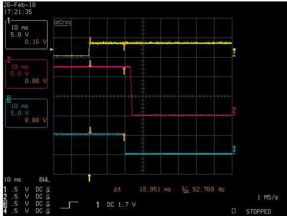
Figure 7: DS1200-3 Turn Off Characteristic via PS_ON Full Load: I_o = 81.7A , I_{SB} = 4A (5V) Ch 1: PS_ON Ch 2: V_o Ch 3: POWER GOOD
