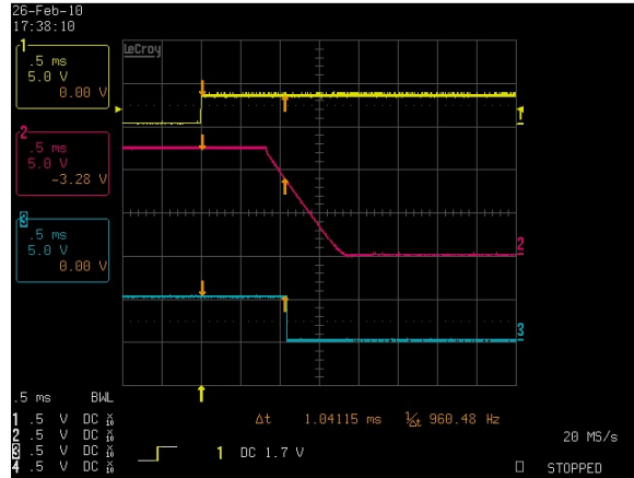
Figure 8: DS1200-3 Turn Off Characteristic via PS_INHIBIT Full Load: I_o = 81.7A , I_{SB} = 4A (5V) Ch 1: PS_INHIBIT Ch 2: V_o Ch 3: POWER GOOD
