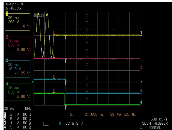
Figure 4: DS1200-3 Hold-up time – V_{IN} = 264\text{Vac} / 47\text{Hz} / 0^\circ Full Load: I_O = 81.7\text{A} , I_{SB} = 4\text{A} (5\text{V})
