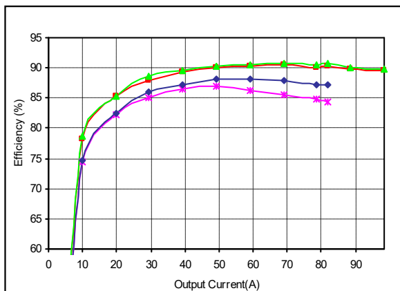
Figure 11: DS1200-3 Efficiency Curves @ 25 degC —●— 80 Vac —■— 115 Vac —▲— 230 Vac —◆— 264 Vac Loading: I_o = 81.7A = 10\% increment to 98.4A, I_{SB} = 0A (5V)
