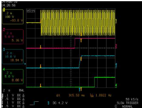
Figure 1: DS1200-3 Turn-on delay via AC mains – V_{IN} = 90\text{Vac}
