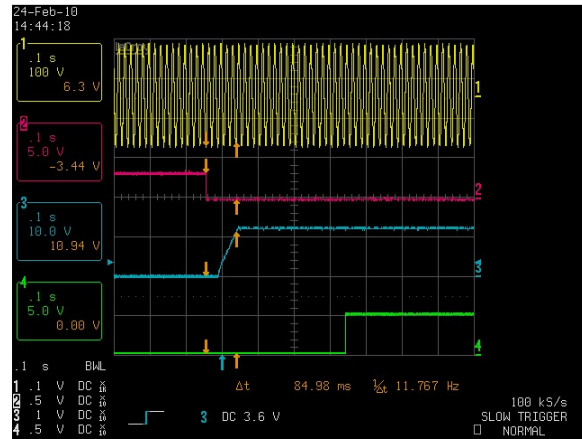
Figure 2: DS1200-3 Turn-on delay via PS_ON – V_{IN} = 90\text{Vac}
