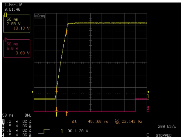
Figure 5: DS1200-3 Output Voltage Startup Characteristic – V_{IN} = 90\text{Vac} Full Load: I_O = 81.7\text{A} , I_{SB} = 4\text{A} (5\text{V})
