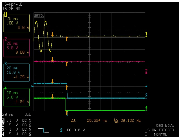
Figure 3: DS1200-3 Hold-up Time – V_{IN} = 90\text{Vac} / 63\text{Hz} / 0^\circ Full Load: I_O = 81.7\text{A} , I_{SB} = 4\text{A} (5\text{V})
