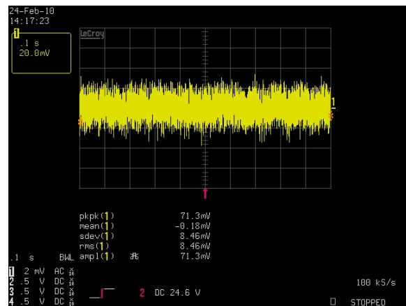
Figure 6: DS1200-3 Ripple and Noise Measurement – V_{IN} = 90\text{Vac} Full Load: I_O = 81.7\text{A} , I_{SB} = 4\text{A} (5\text{V})
